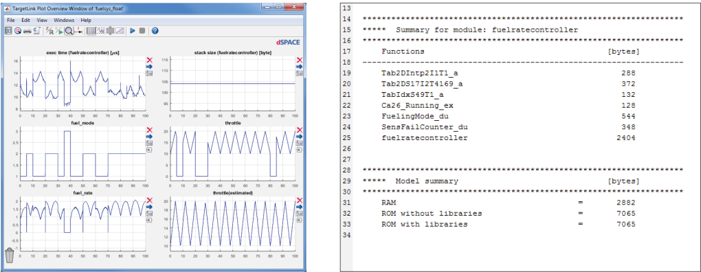
Results from PIL simulation (left) and code summary (right).
