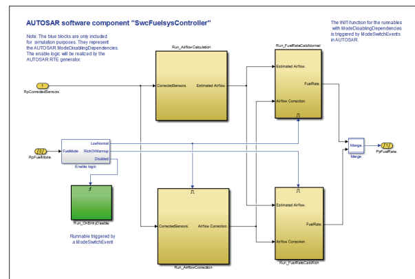
Modeling Classic AUTOSAR SWCs.
