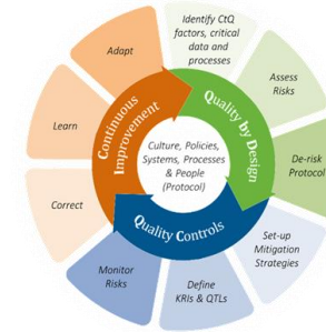
Risk-Based CDM
